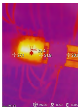
Electric switch
